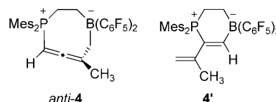
Scheme 2. Possible isomeric addition products, anti - 4 and 4' .
